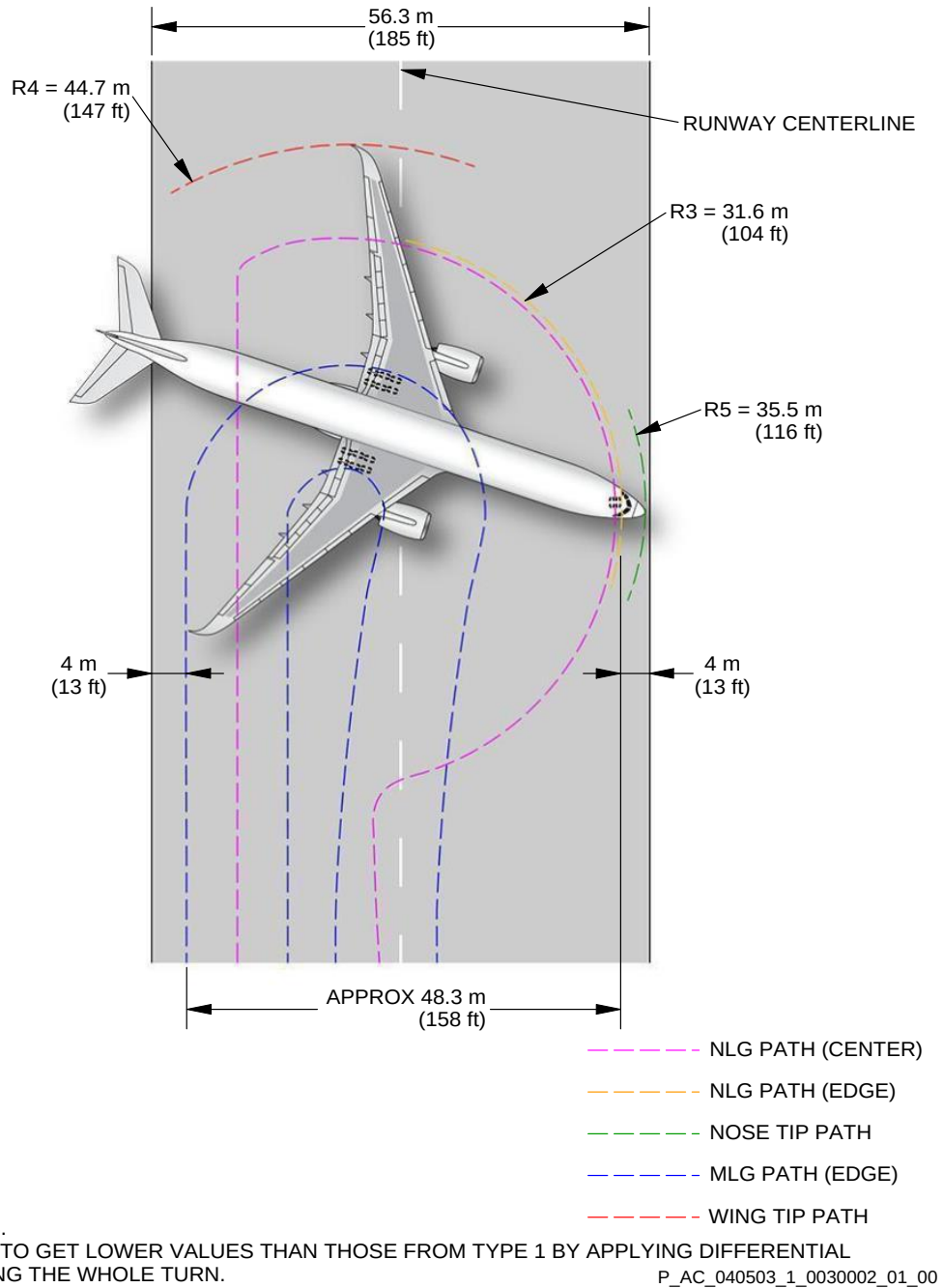
180° Turn on a Runway FIGURE-4-5-3-991-003-B01
