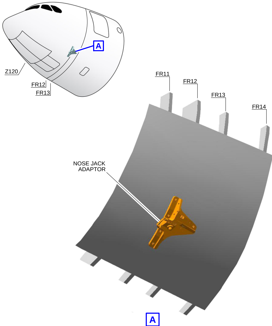
Jacking for Maintenance (Sheet 3 of 5) FIGURE-2-14-1-991-007-A01
