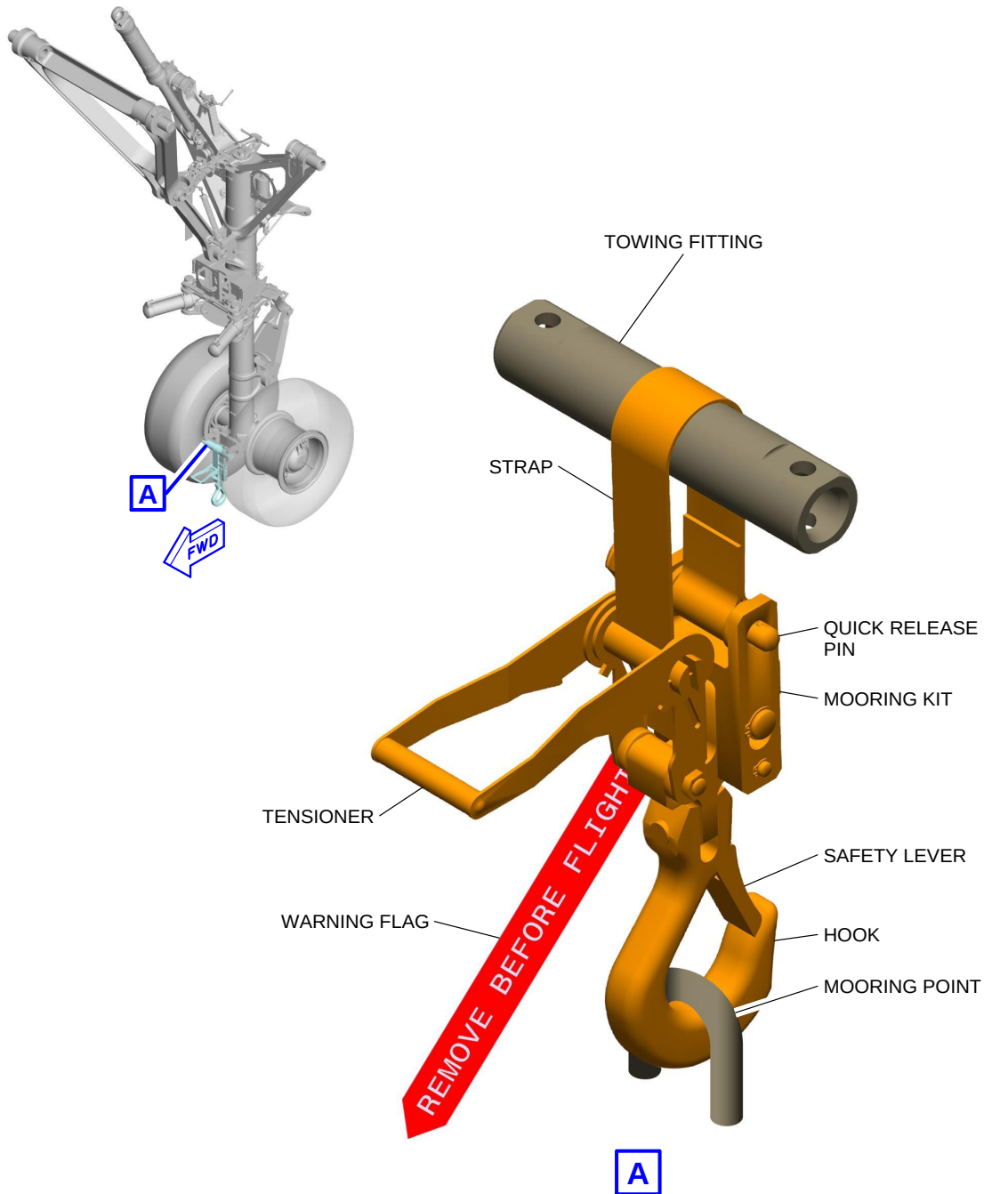
Aircraft Mooring FIGURE-4-8-0-991-001-A01
