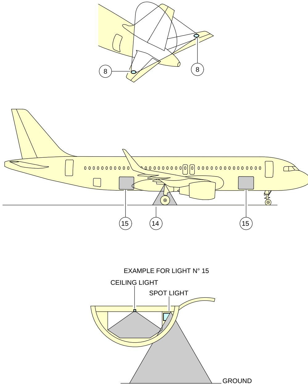
Exterior Lighting FIGURE-2-10-0-991-019-A01
