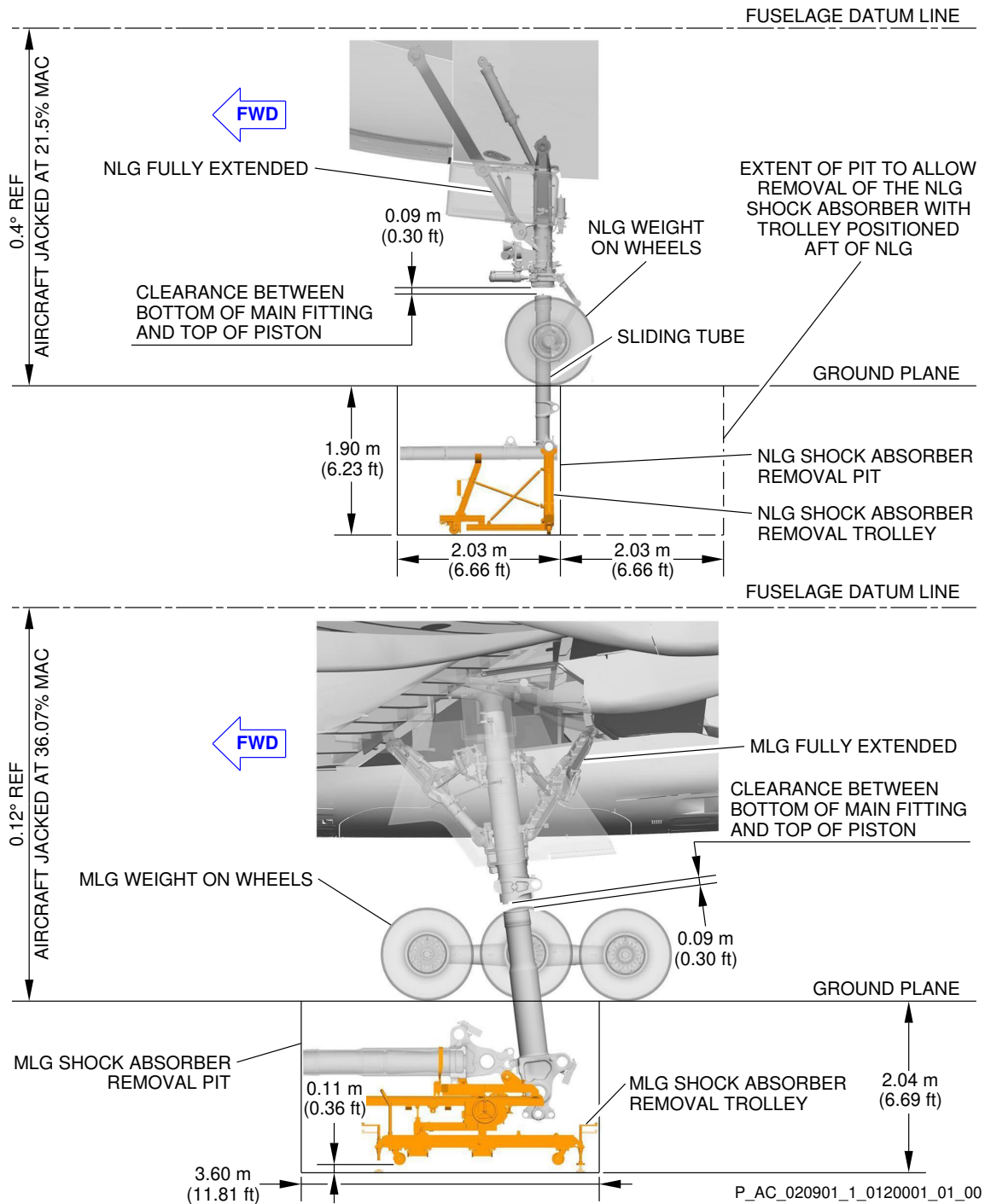
NLG/MLG Shock Absorber Removal Pit FIGURE-2-9-1-991-012-A01
