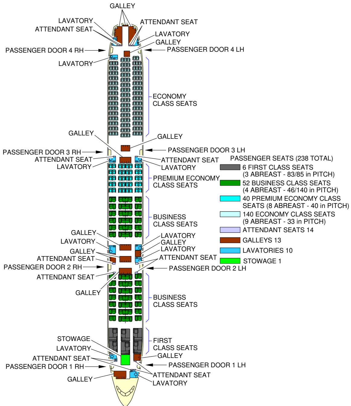
Standard Configuration Standard Configuration (ULR) (Sheet 3 of 3) FIGURE-2-4-0-991-002-A01
