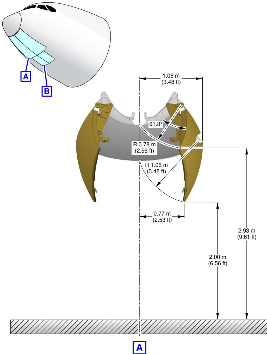
Nose Landing Gear Doors (Sheet 1 of 2) FIGURE-2-7-0-991-131-A01
