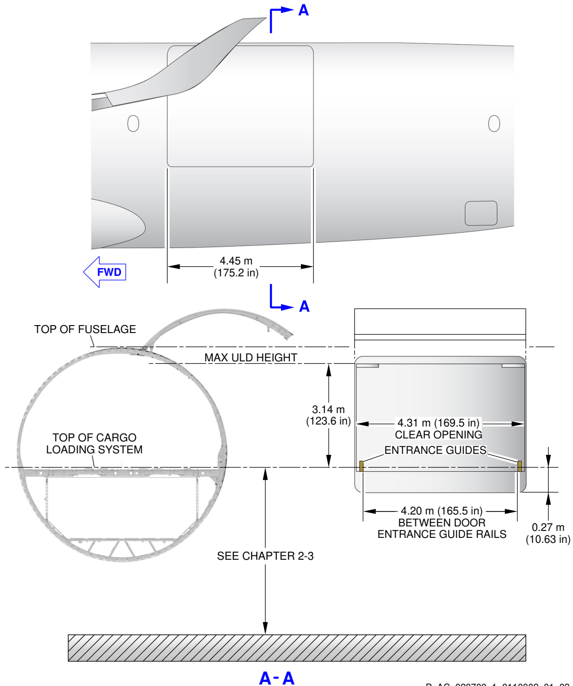
Main Deck Cargo Door FIGURE-2-7-0-991-011-B01
