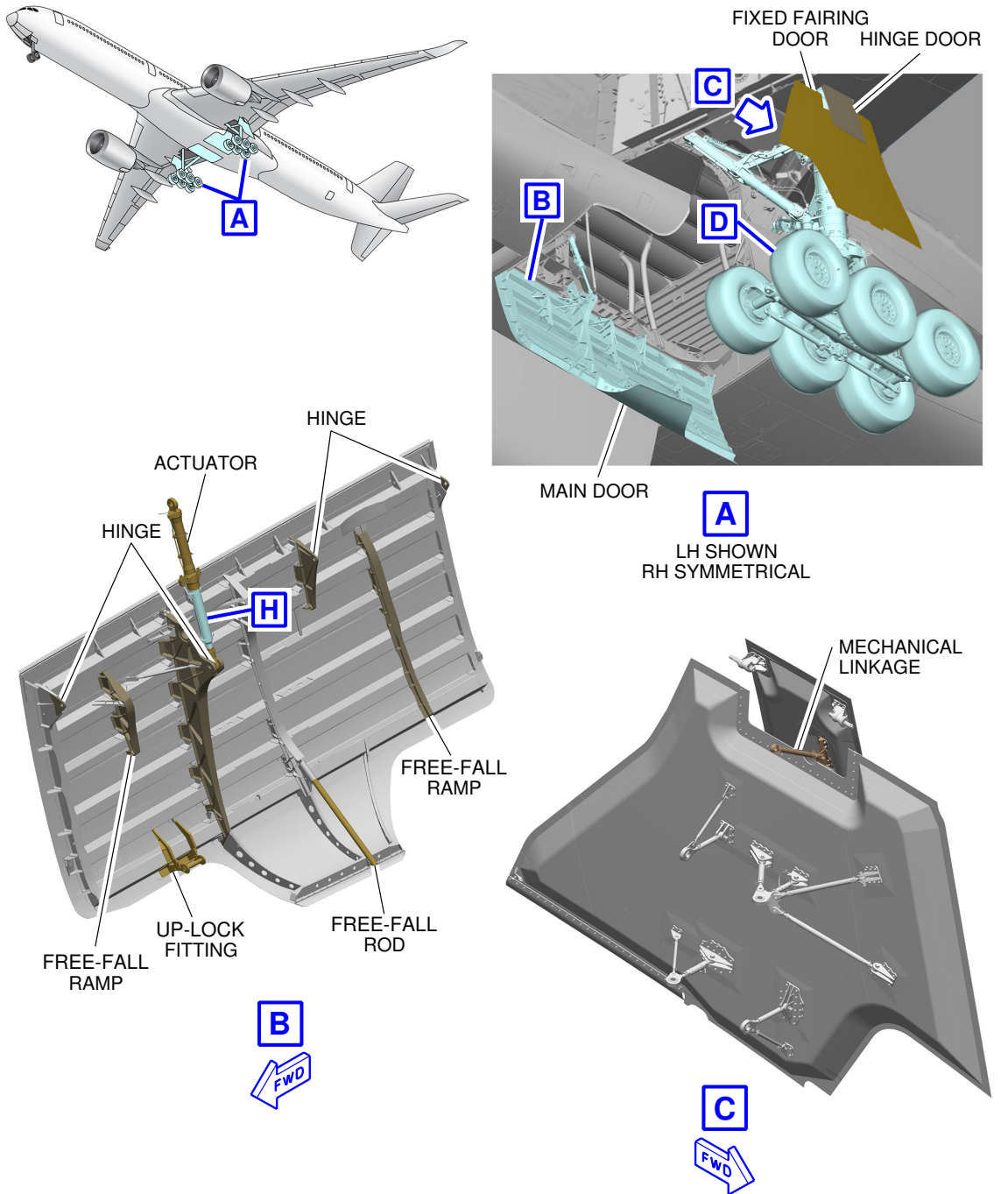
Main Landing Gear Doors Overview (Sheet 1 of 3) FIGURE-2-9-0-991-001-B01
