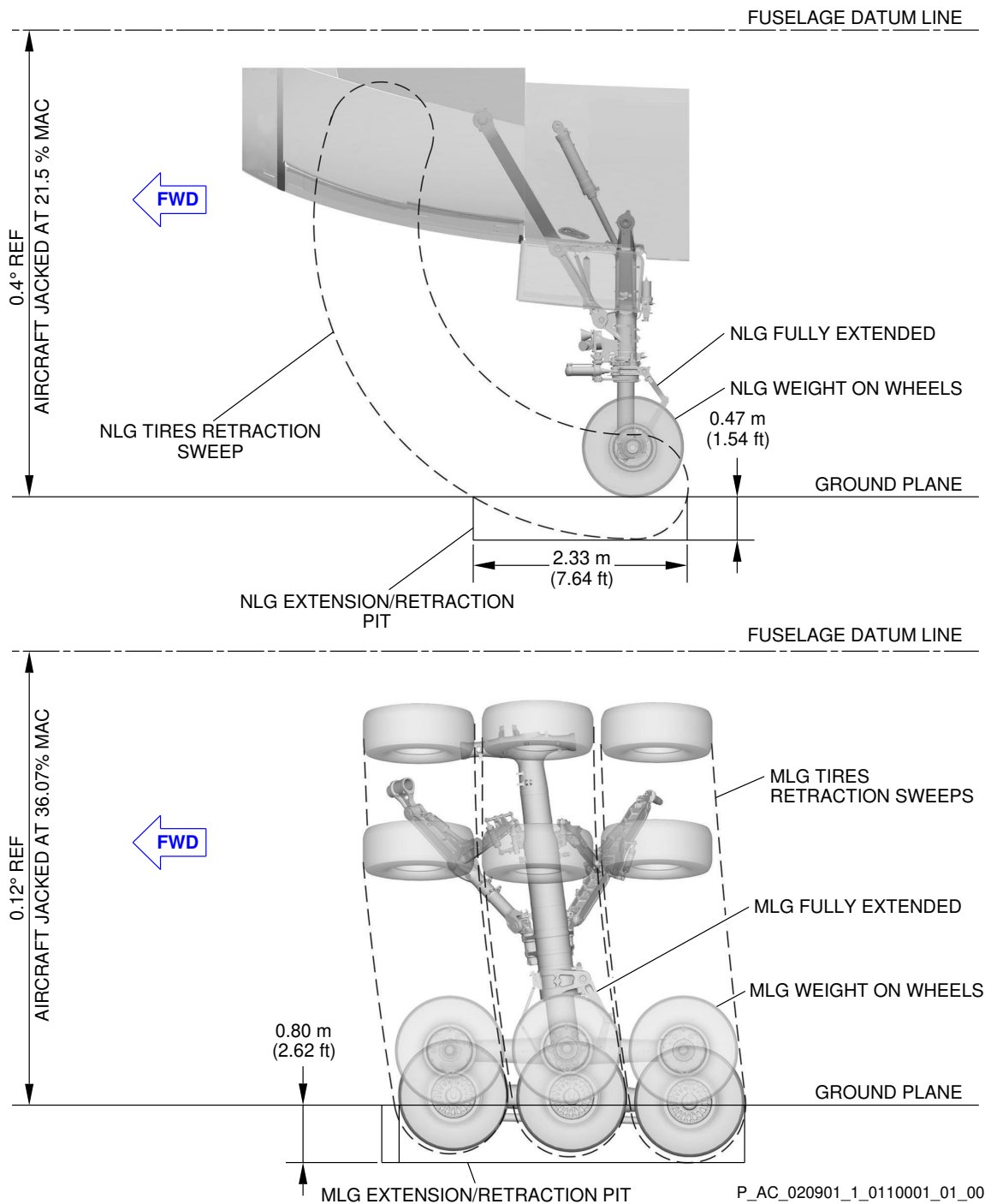
NLG/MLG Extension/Retraction Pit FIGURE-2-9-1-991-011-A01
