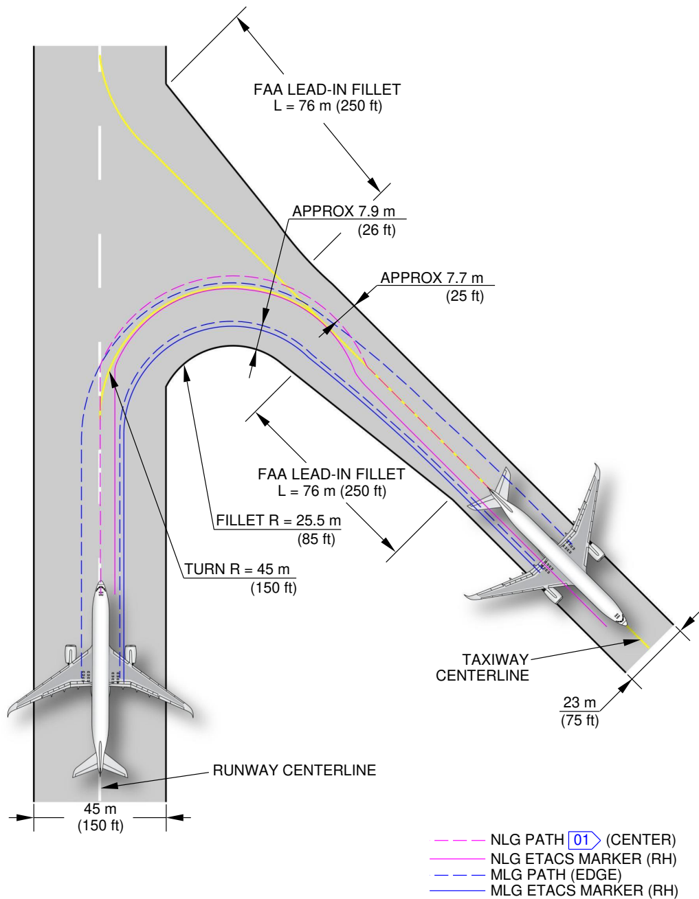
135° Turn - Runway to Taxiway ETACS Assisted Steering Method (Sheet 2 of 3) FIGURE-4-5-1-991-001-A01
