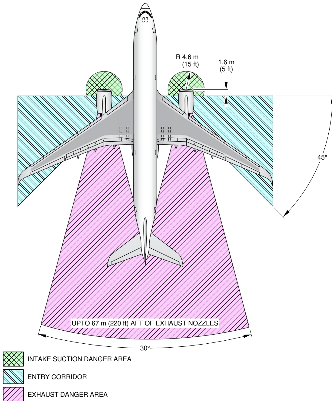
Ground Idle Power - TRENT XWB-84 Engine FIGURE-6-3-1-991-001-A01
