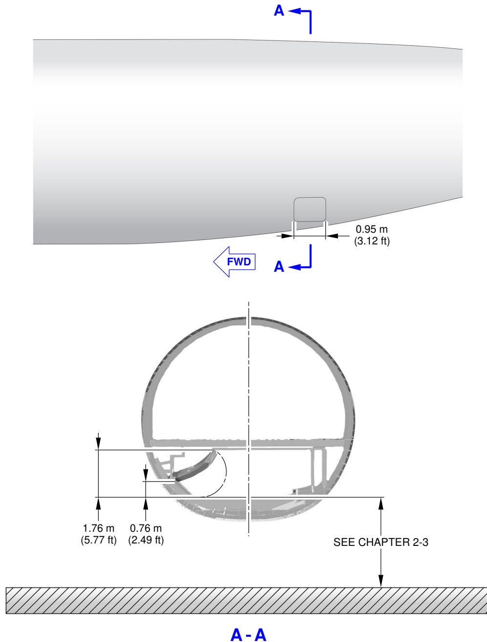
Bulk Cargo Compartment Door FIGURE-2-7-0-991-101-A01
