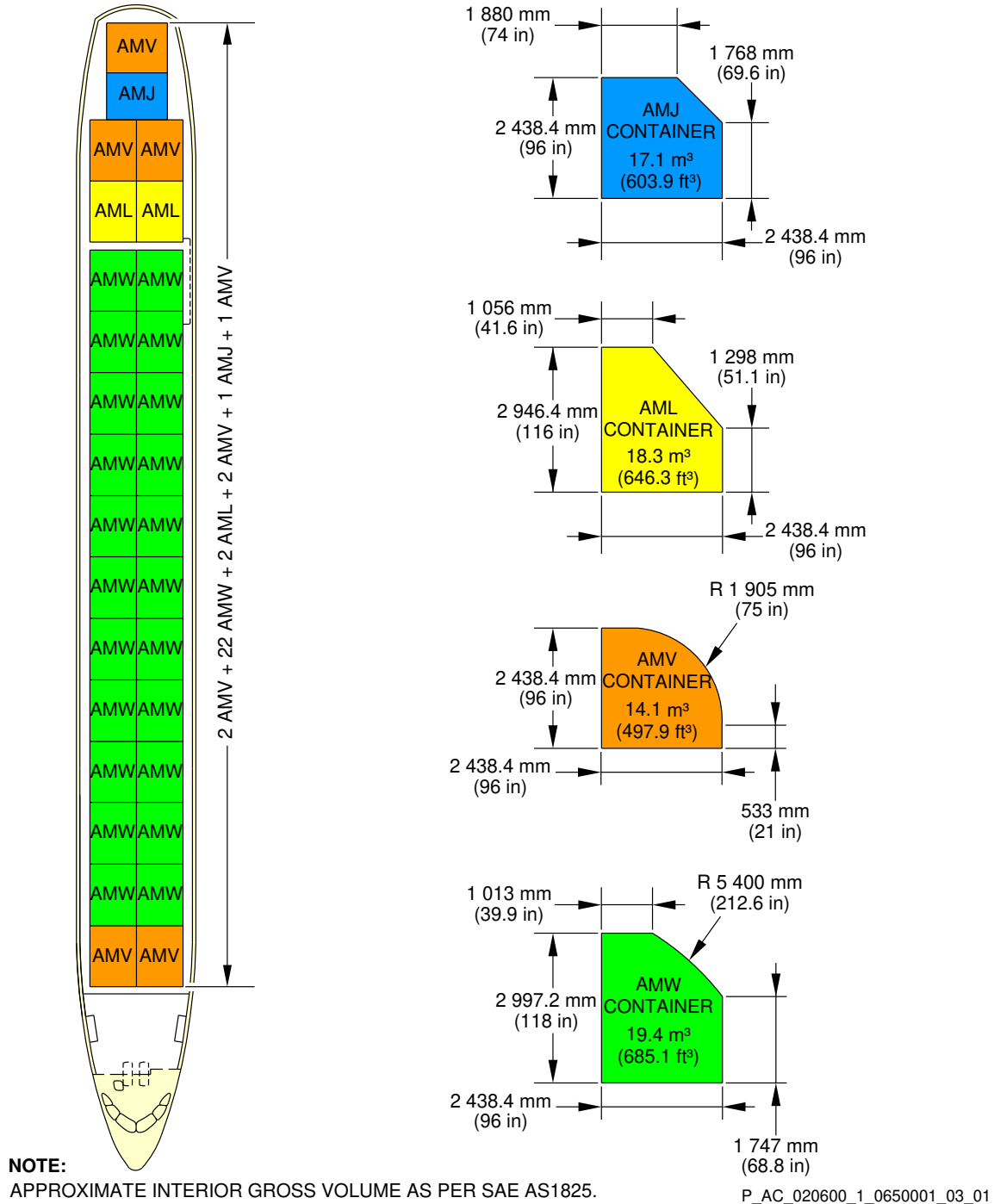
Main Deck Cargo Compartment (Sheet 3 of 3) FIGURE-2-6-0-991-065-A01
