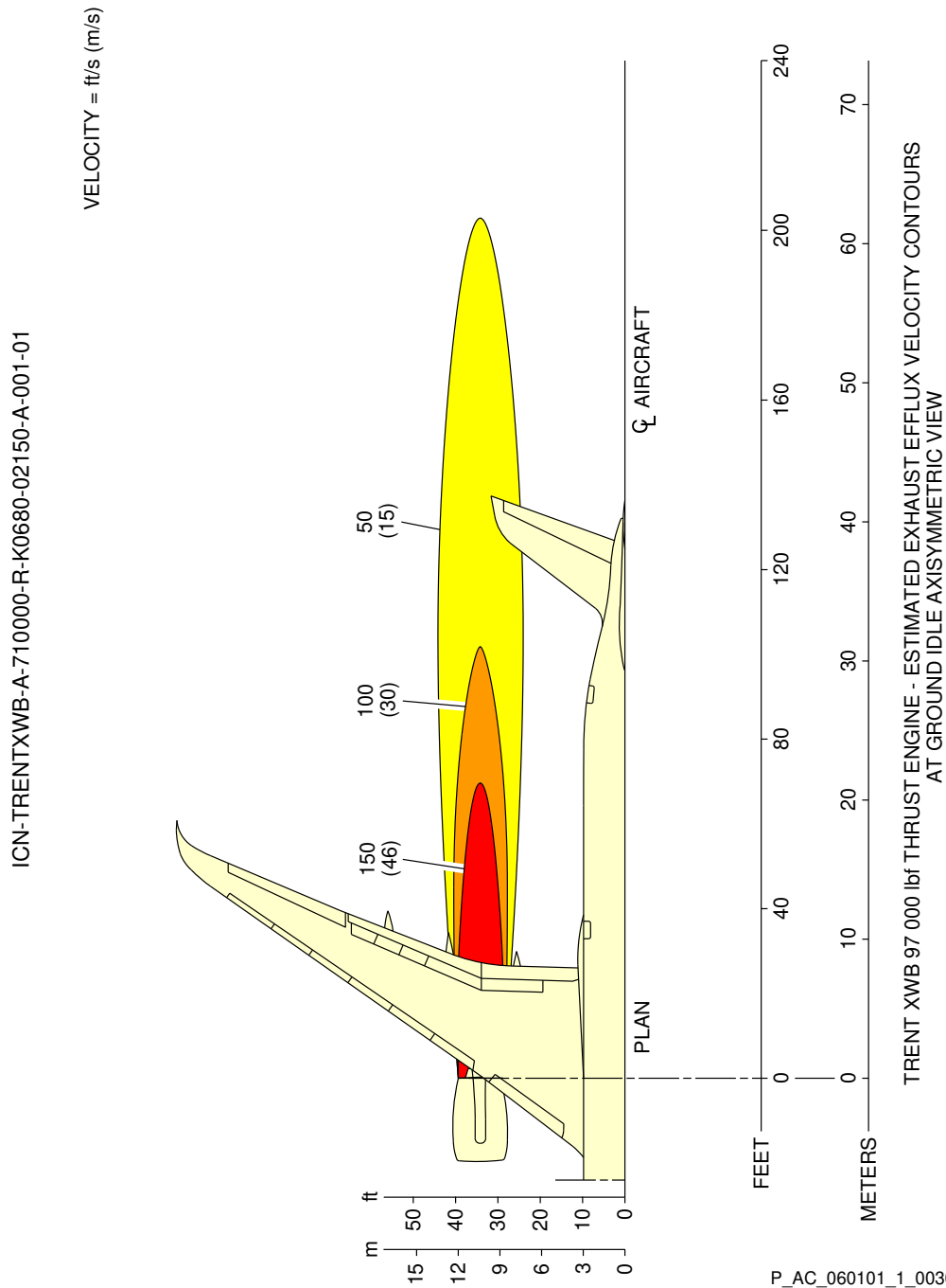
Ground Idle Power - TRENT XWB-97 Engine FIGURE-6-1-1-991-003-A01
