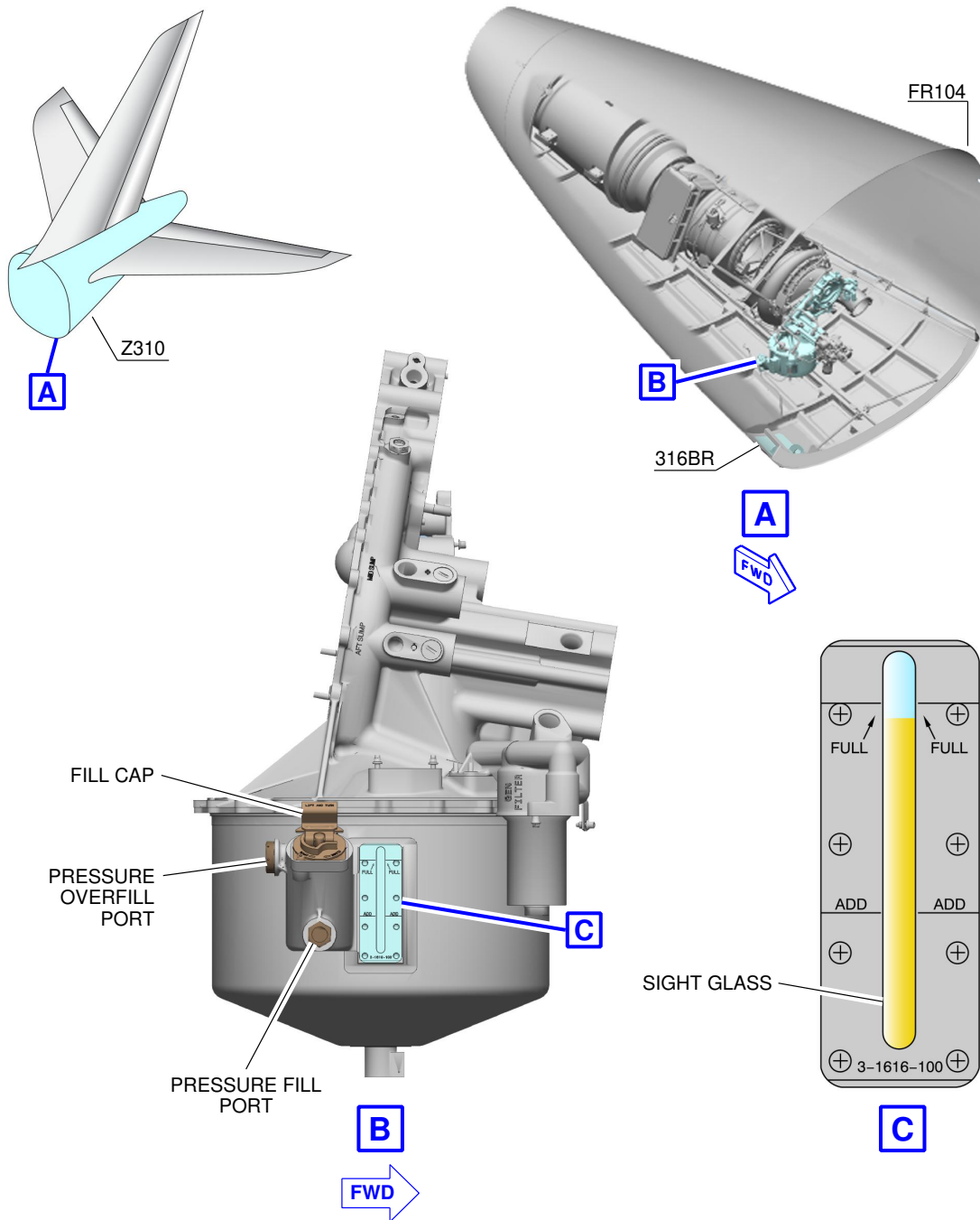
APU Oil Servicing FIGURE-5-4-7-991-011-A01
