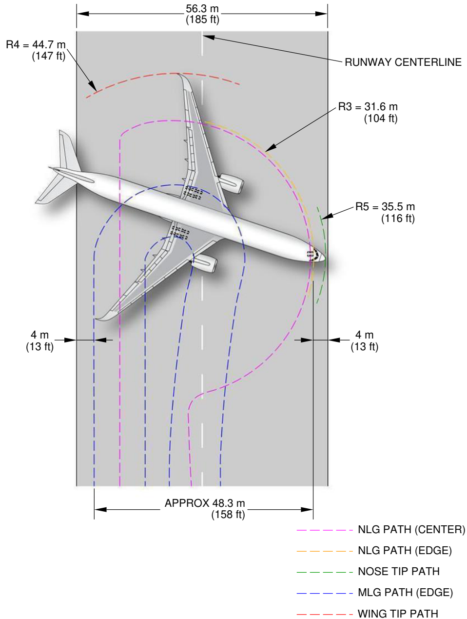
180° Turn on a Runway FIGURE-4-5-3-991-003-B01
