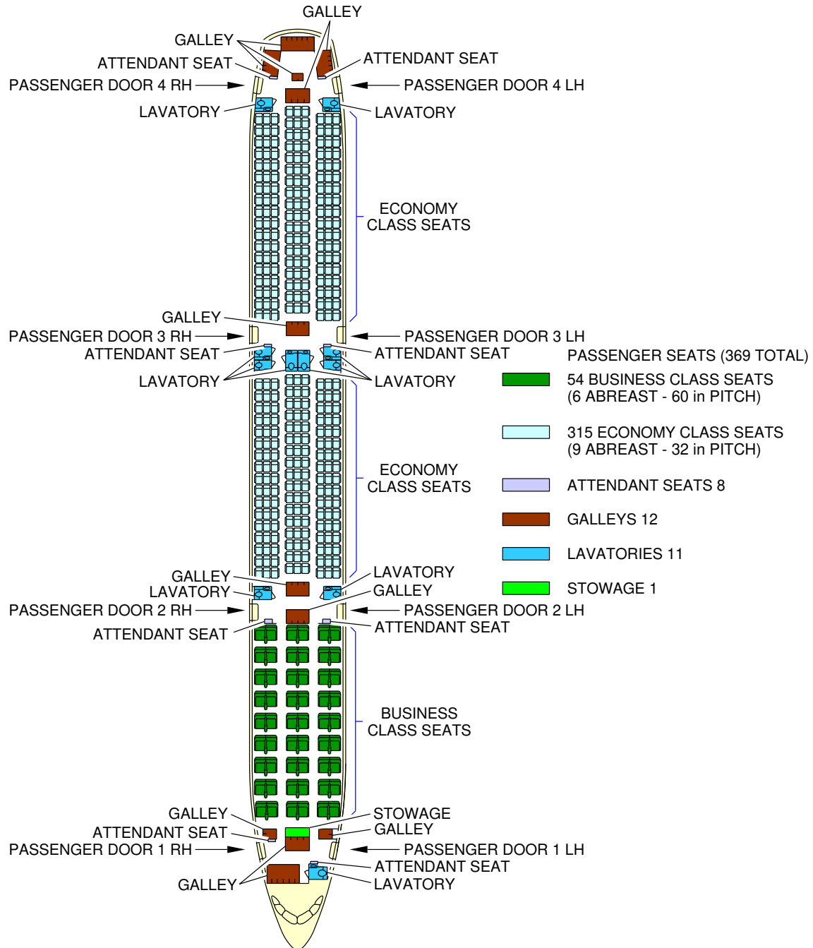
Standard Configuration (Sheet 1 of 3) FIGURE-2-4-0-991-002-A01
