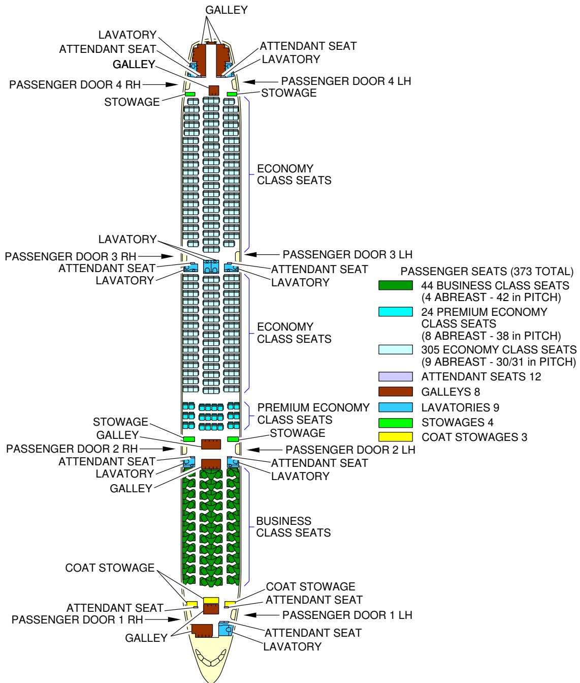
Standard Configuration (Sheet 2 of 3) FIGURE-2-4-0-991-002-A01
