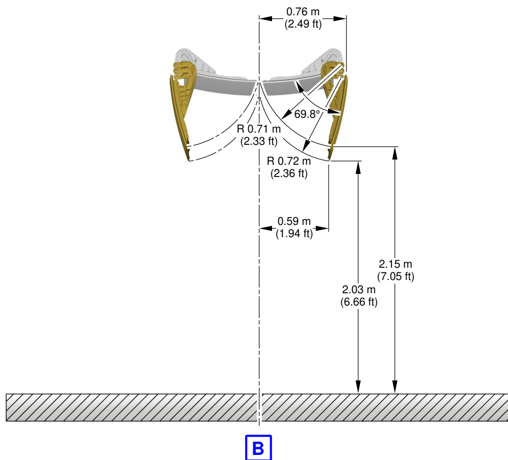
Nose Landing Gear Doors (Sheet 2 of 2) FIGURE-2-7-0-991-131-A01
