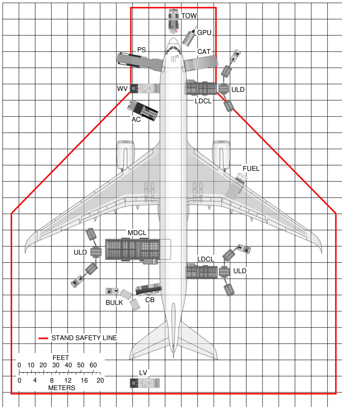
Typical Ramp Layout (Open Apron) FIGURE-5-1-1-991-004-A01
