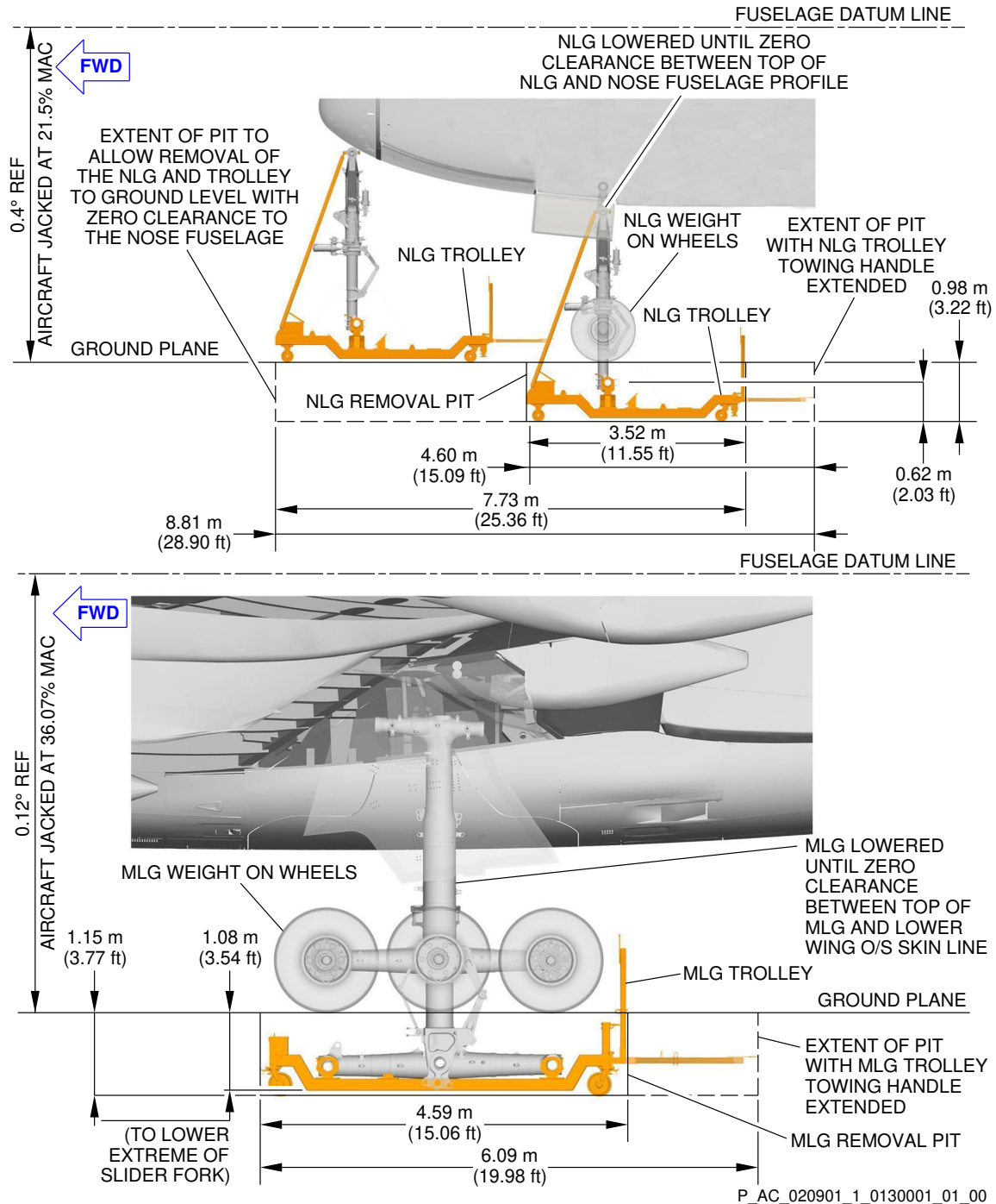
NLG/MLG Removal Pit FIGURE-2-9-1-991-013-A01
