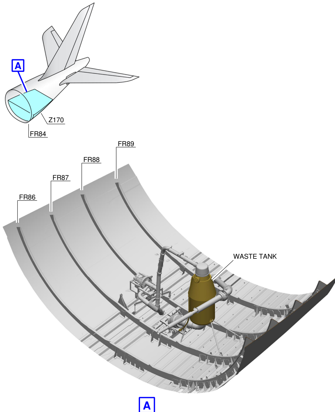
Waste Tanks Location FIGURE-5-4-9-991-002-C01
