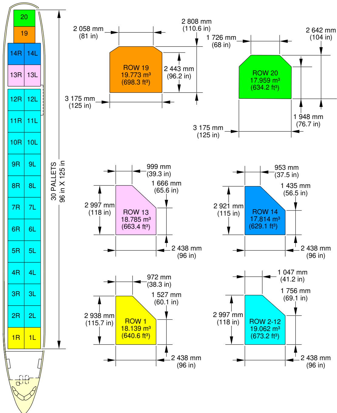
Main Deck Cargo Compartment (Sheet 2 of 3) FIGURE-2-6-0-991-065-A01
