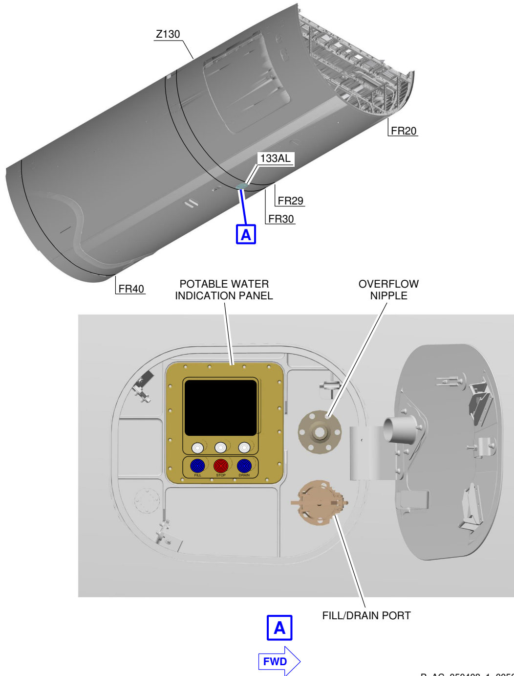
Potable-Water Ground Service Panel FIGURE-5-4-8-991-005-E01
