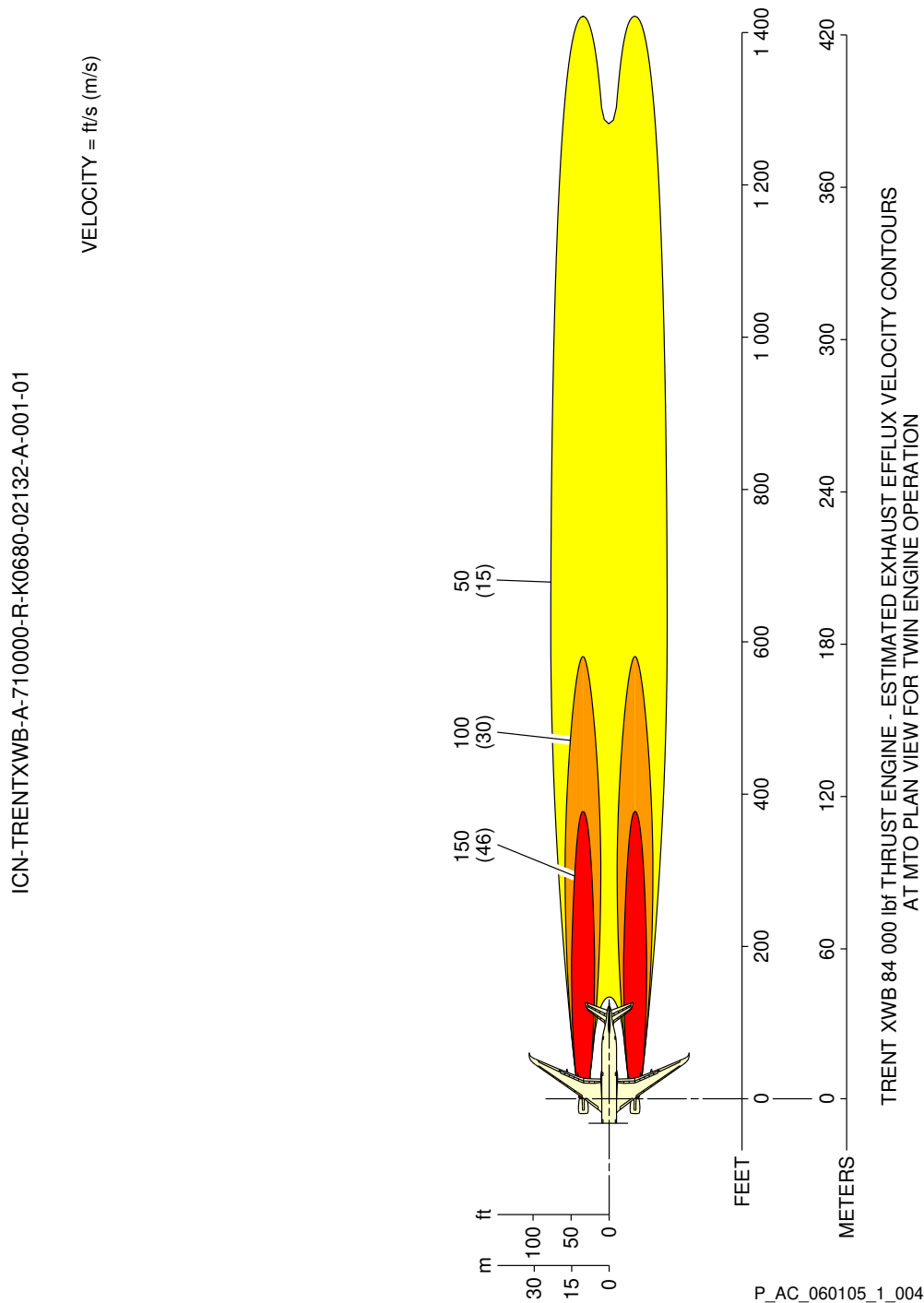
Max Take-Off Power - TRENT XWB-84 Engine (Sheet 2 of 2) FIGURE-6-1-5-991-004-A01
